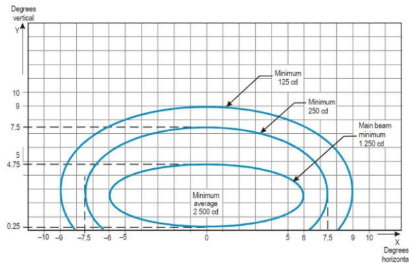
ICAO requirements Annex 14 Vol.1 Fig. A2-8. RED
